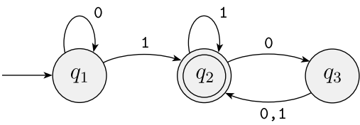
FIGURE 1.6 The finite automaton M_1
