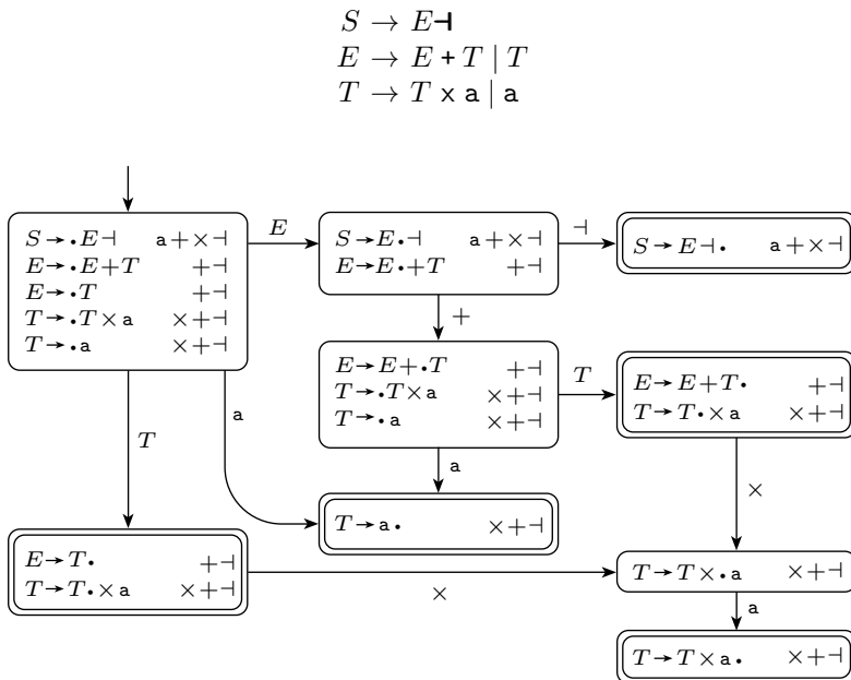
FIGURE 2.65 Passing the DK_1 -test
