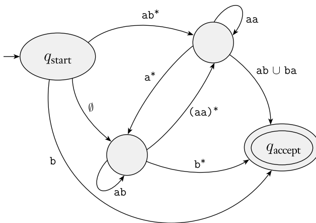
FIGURE 1.61 A generalized nondeterministic finite automaton
