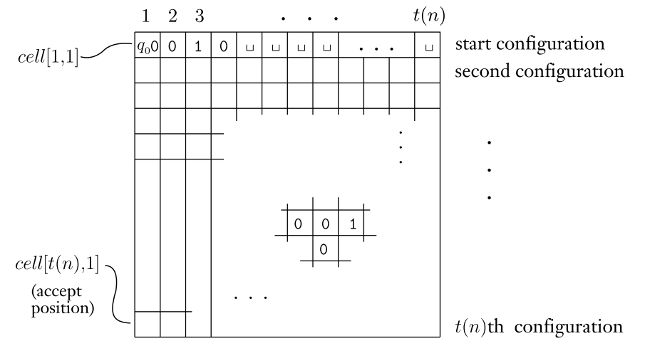
FIGURE 9.31 A tableau for M on input 0010
