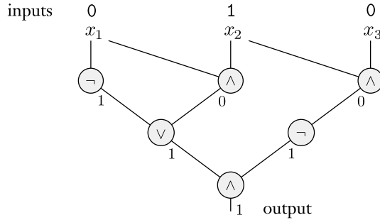
FIGURE 9.24 An example of a Boolean circuit computing
