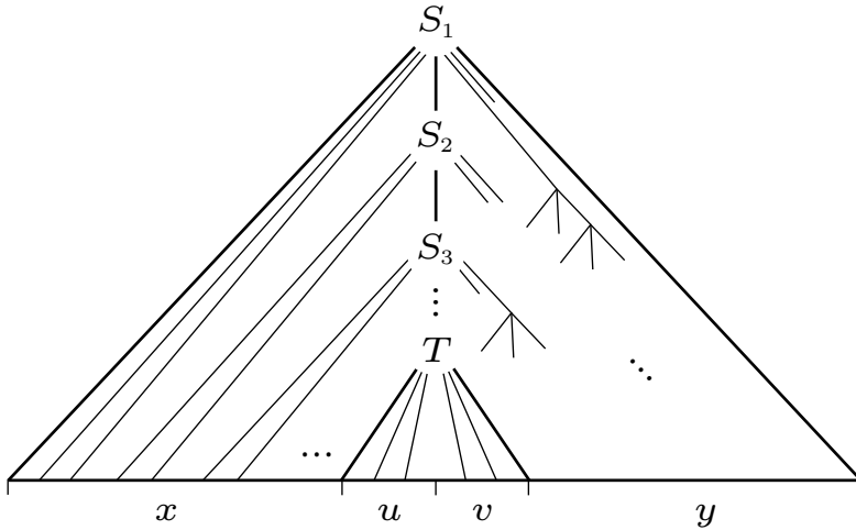
FIGURE 2.50 Parse tree leading to valid string xuvy with handle uv
