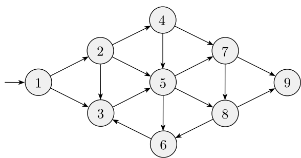
FIGURE 8.13 A sample generalized geography game
