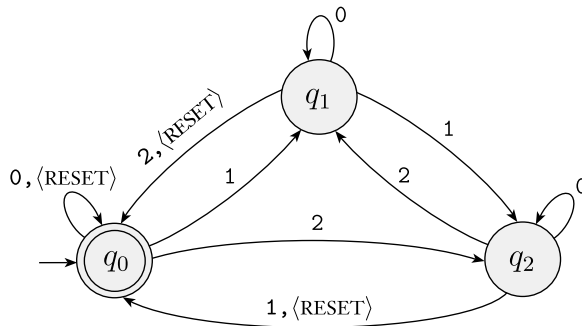
FIGURE 1.14 Finite automaton M_5
