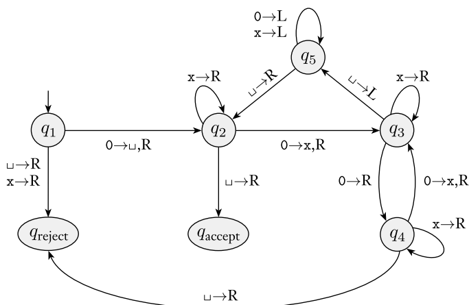
FIGURE 3.8 State diagram for Turing machine M_2
